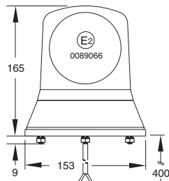
MOUNTING BOLT ARRANGEMENT
