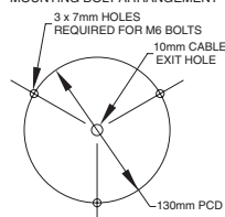
MOUNTING BOLT ARRANGEMENT
