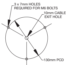
MOUNTING BOLT ARRANGEMENT
