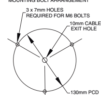
MOUNTING BOLT ARRANGEMENT
